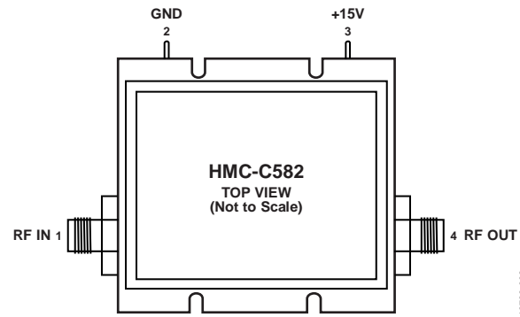
Figure 2. Pin Configuration
